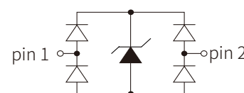
Schematic Symbol
