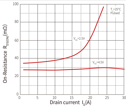
Figure 3: R_{DS(ON)} - I_D
