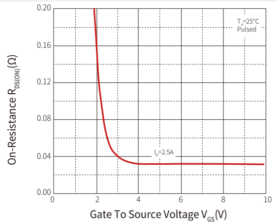
Figure 4: R_{DS(ON)} - V_{GS}
